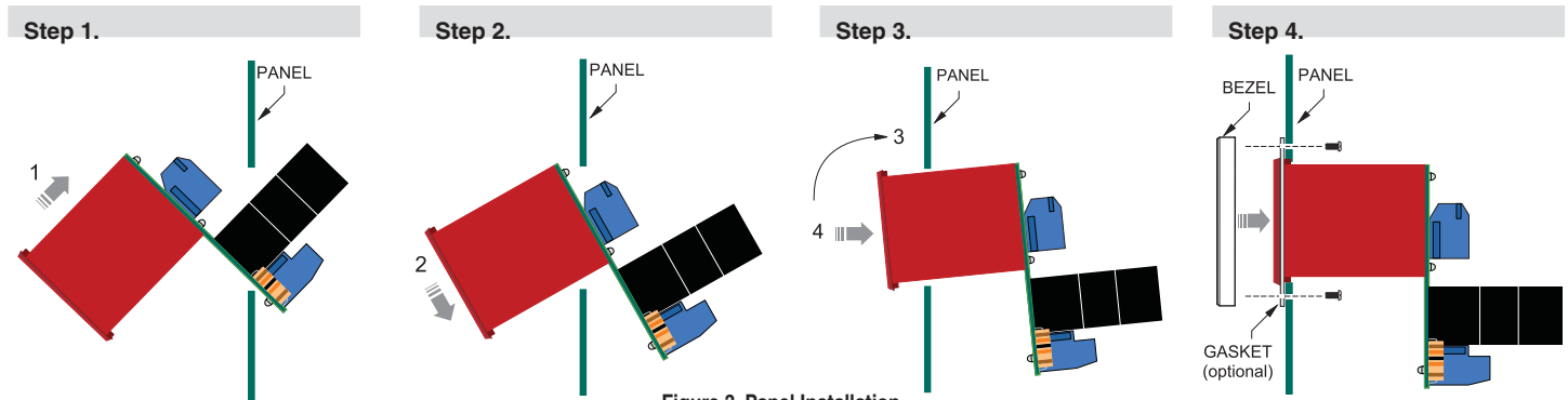
Figure 3. Panel Installation
