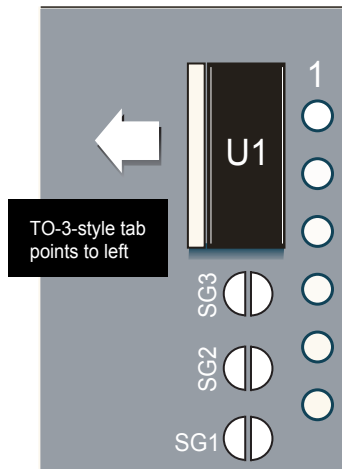
Figure 3. Installing U1
