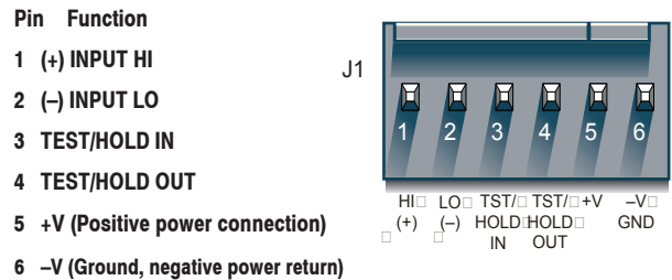
Figure 2. J1 Connector Pinout
