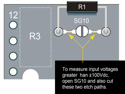
Figure 4. Installing R1
