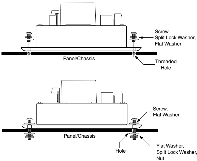
Figure 4. Chassis Mounting
